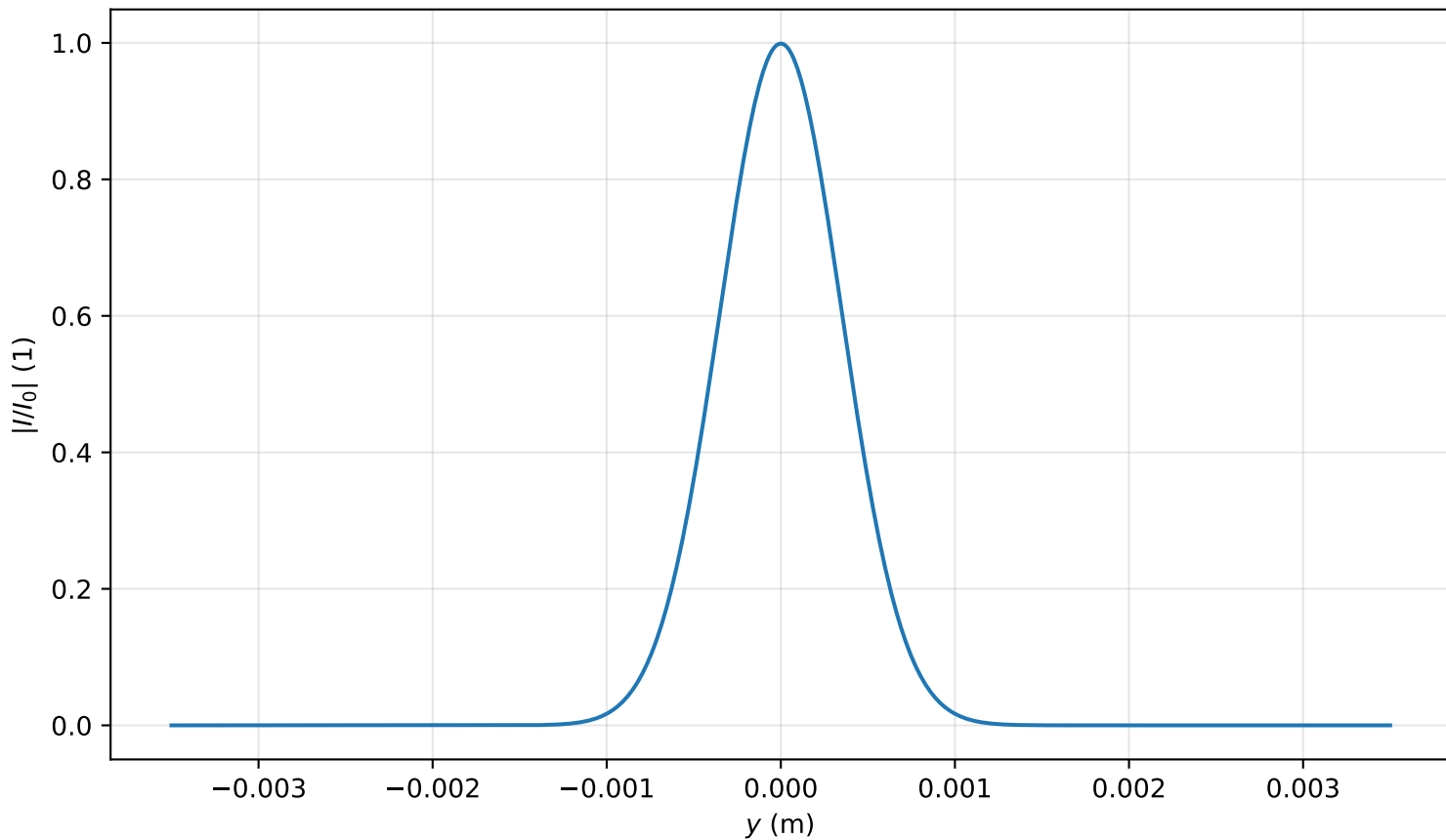
Intensity profile I(x = 0, y, z = 0.080)/I_0 , \text{Pin}=0.1\text{Pcr} , artificial time
